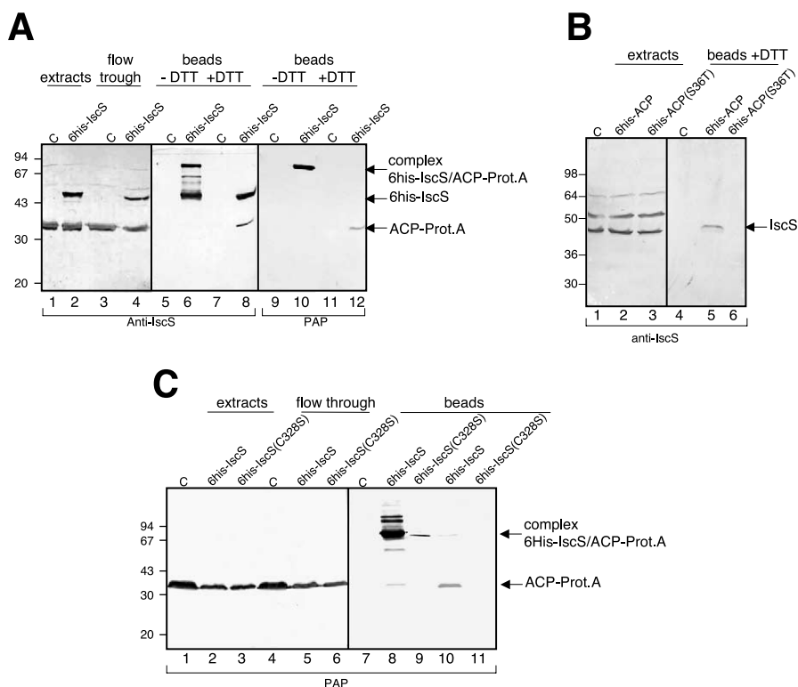
Fig. 3. ACP is linked to IscS by a disulfide bond. Cultures were induced for 60 min with 0.01% arabinose at OD_{600nm}=0.8 at 37°C. Final OD_{600nm} was approximately 2. Extracts were done in buffer 1 without reducing agent (20 mM Tris-HCl pH 8.0, 200 mM NaCl, 0.2% NP40, 10 mM imidazole) at a concentration of 50 uOD_{600nm}/ml by sonication. 30 \mu l of cobalt beads were used for each test with 1 ml of extract. Elution was done in Laemmli loading buffer without or with 2 mM DTT. A: Co-precipitation of ACP-Prot.A with 6His-IscS. In this experiment, both ACP-Prot.A and 6His-IscS expressions were induced by arabinose. Lanes 1 and 2: extracts; lanes 3 and 4: flow through; lanes 5,6,9 and 10: beads without DTT; lanes 7,8,11 and 12: beads with 2 mM DTT added after elution; odd lanes: control ACP-Prot.A/W3110; even lanes: 6His-IscS/ACP-Prot.A/W3110. Samples were analyzed by 12% SDS-PAGE and Western blot with an anti-IscS antibody (lanes 1–8) or a PAP antibody detecting the Prot.A tag (lanes 9–12). Using the anti-IscS antibody, ACP-Prot.A was also detected in lanes 1–8 owing to the fixation of any antibodies to the Prot.A tag. B: IscS does not co-precipitate with 6His-ACP(Ser36Thr). Lanes 1–3: extracts; lanes 4–6: beads treated with DTT; lanes 1 and 4: control W3110; lanes 2 and 5: 6His-ACP/W3110; lanes 3 and 6: 6His-ACP(Ser36Thr)/W3110. Samples were analyzed by 10% SDS-PAGE and Western blot with an anti-IscS antibody. C: ACP-Prot.A does not bind to 6His-IscS(Cys328Ser). Lanes 1–3: extracts; lanes 4–6: flow through; lanes 7–9: beads without added DTT; lanes 10–11: beads with 2 mM DTT after elution; lanes 1, 4, and 7: control ACP-Prot.A/W3110; Lanes 2,5,8 and 10: 6His-IscS/ACP-Prot.A/W3110. lanes 3, 6, 9, and 11: 6His-IscS(Cys328Ser)/ACP-Prot.A/W3110. Samples were analyzed by 10% SDS-PAGE and Western blot with PAP antibody.
